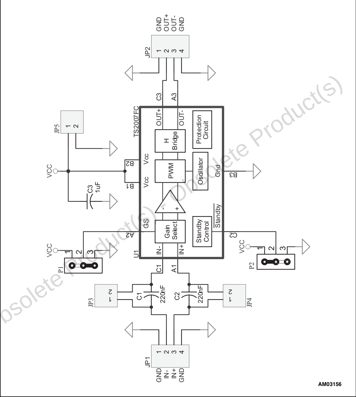
Figure 1. Schematic diagram
